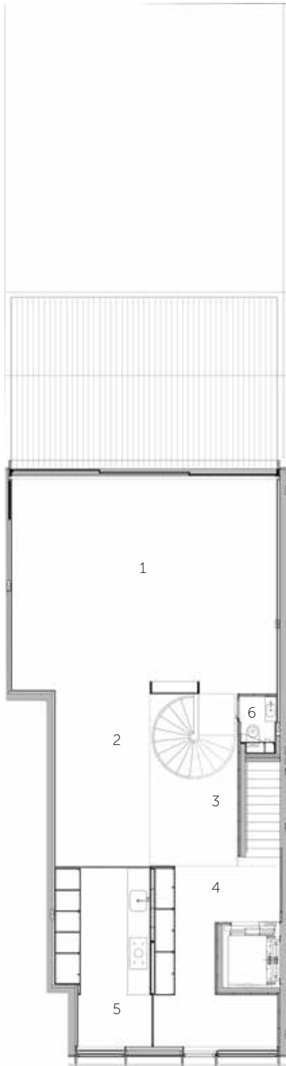
FLOOR 0
