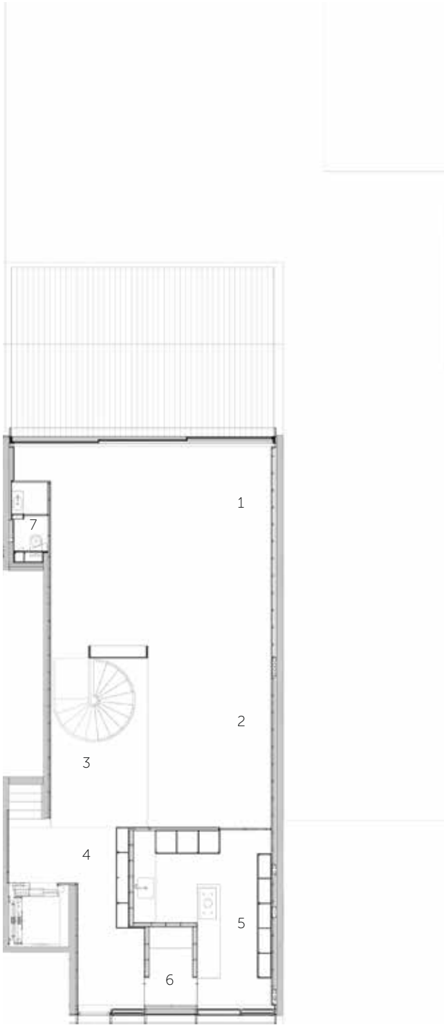
FLOOR 0
