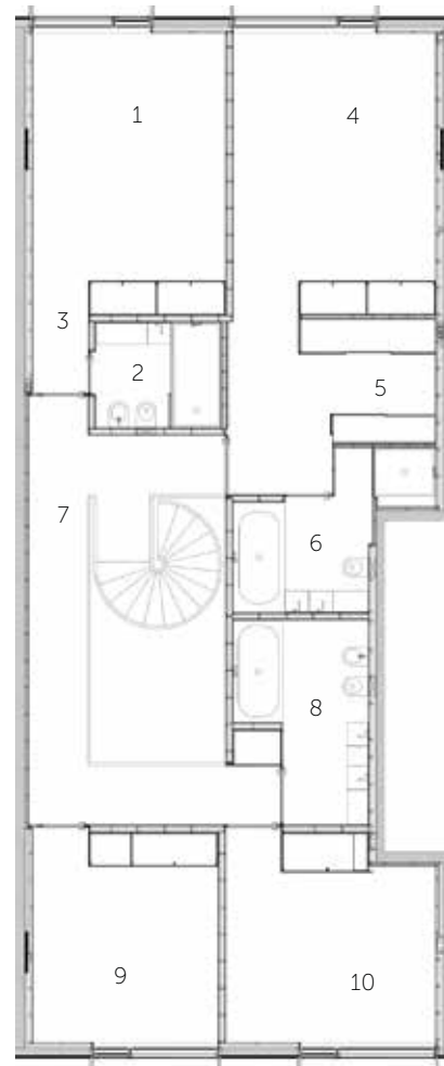
FLOOR 1
