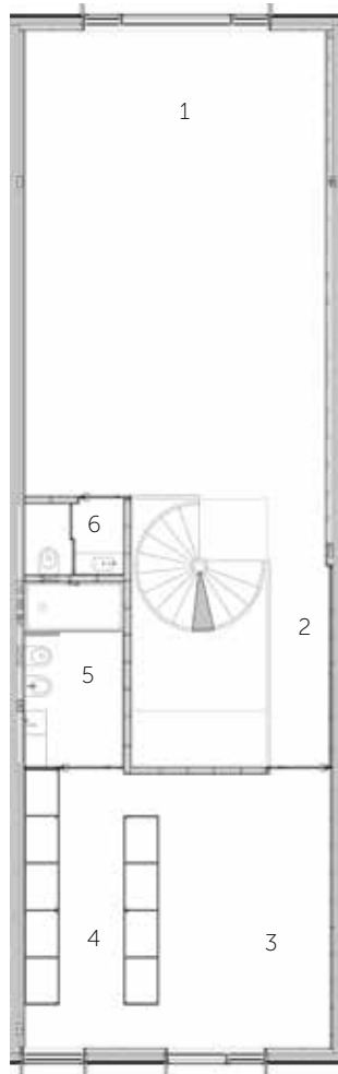
FLOOR 1
